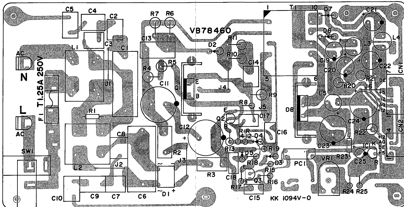
<Components side>
